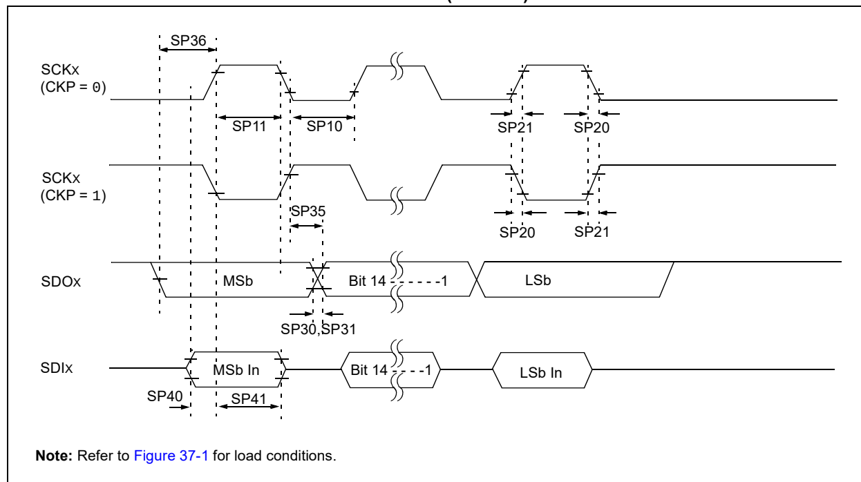
FIGURE 37-11: SPIx MODULE MASTER MODE (CKE = 1) TIMING CHARACTERISTICS
